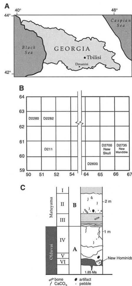
Fig. 1. (A) Location map of Dmanisi site. (B) The locations of hominid fossils (excavation units are 1-m squares). (C) General stratigraphic profile, modified after Gabunia et al. (5, 6). The basalt and the immediately overlying volcanoclastics (stratum A) exhibit normal polarity and are correlated with the terminus of the Olduvai Subchron. Slightly higher in the section, above a minor disconformity and below a strongly developed soil, Unit B deposits, which also contain artifacts, faunas and human fossils, all exhibit reversed polarity and are correlated with the Matuyama. Even the least stable minerals, such as olivine, in the basalt and the fossil-bearing sediments show only minor weathering, which is compatible with the incipient pedogenic properties of the sediments.
